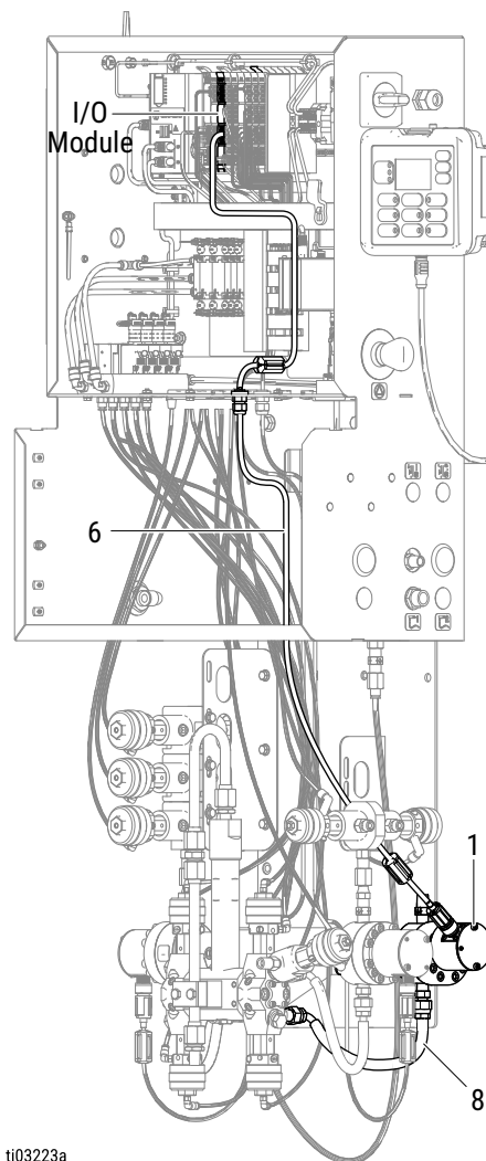
FIG. 1: Package Meter Proportioner Typical Installation
