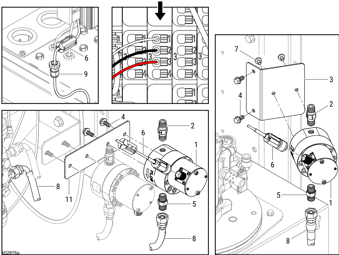
ProMix V Package Meter Proportioner
